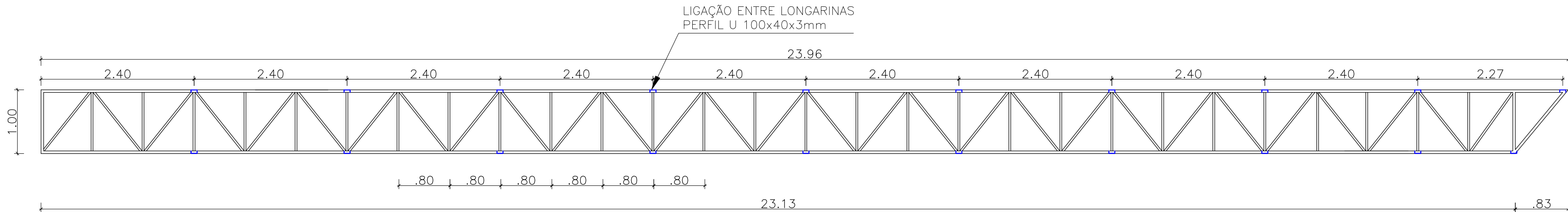
LOGONGARINA (02 UND)
