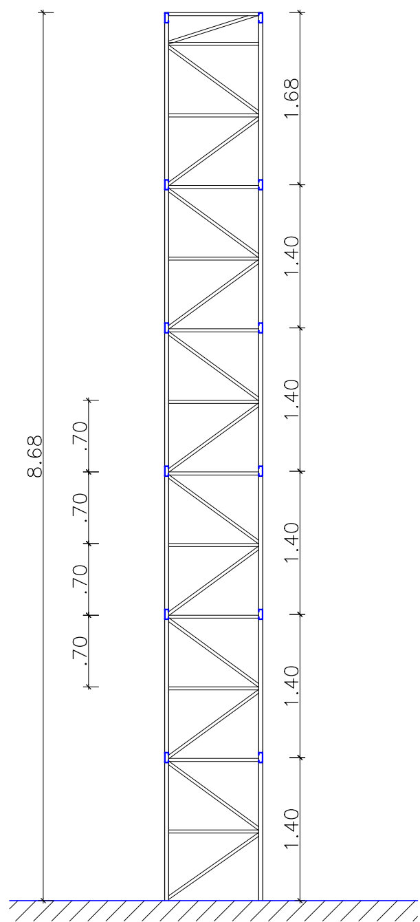
PILAR 01 (08 UND)
