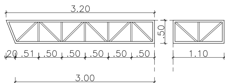
VIGA 02 (02 UND)
